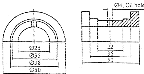
CASTING, C.I. 1 OFF
